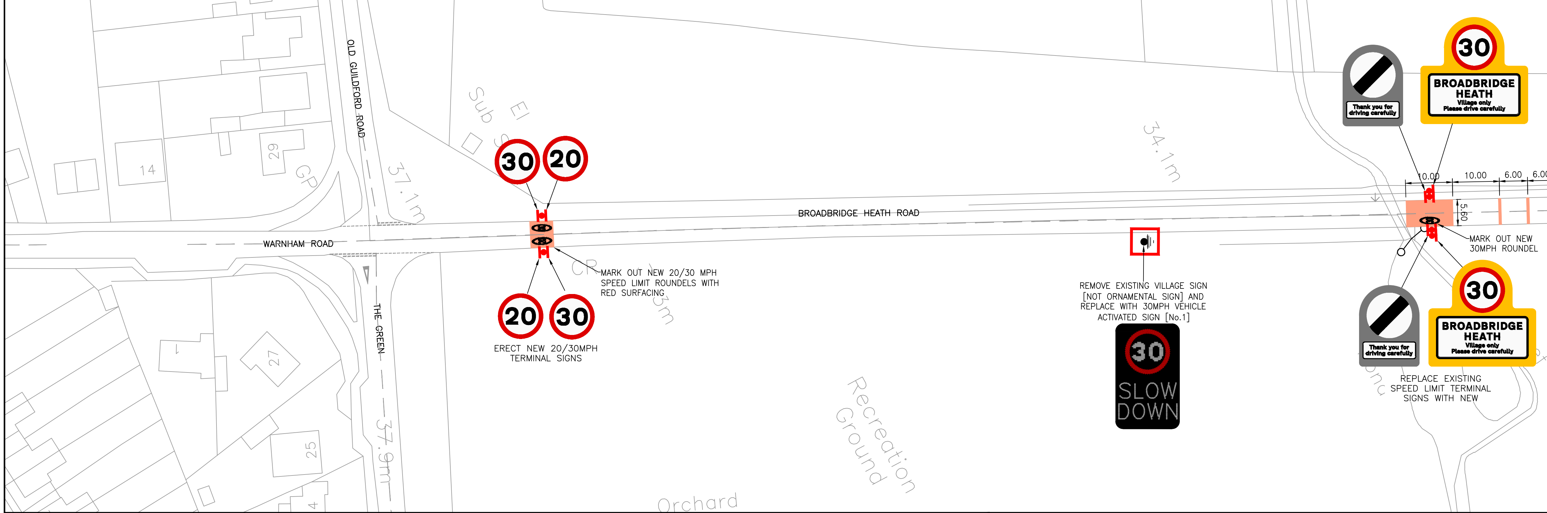
DETAIL A BROADBRIDGE HEATH ROAD - GATEWAY FEATURES SCALE 1:500
